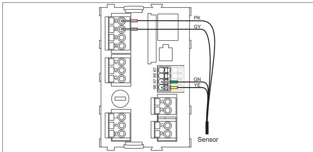
Fig. 15: Sensor connection
