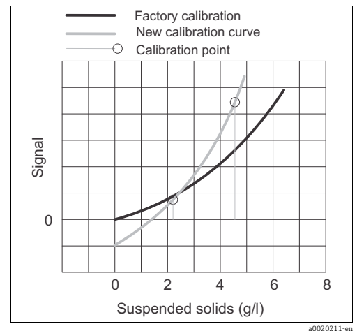
Fig. 24: Two-point calibration
