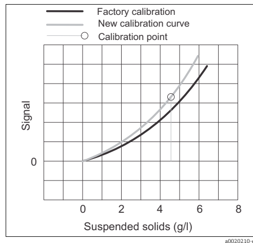
Fig. 23: Single-point calibration
