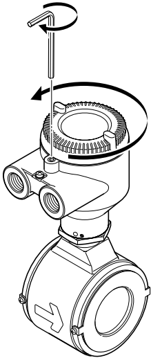
Figure 4.2.8 Removing the Terminal Box Cover (Remote Flowtube)
