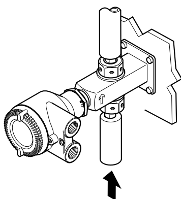
Vertical mounting
