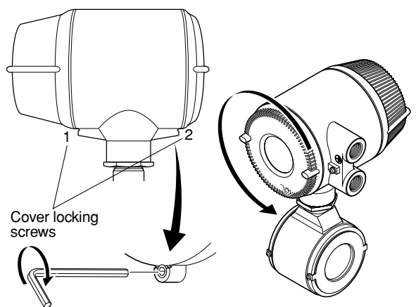
Figure 4.1.5 Removing the Terminal Box Cover
