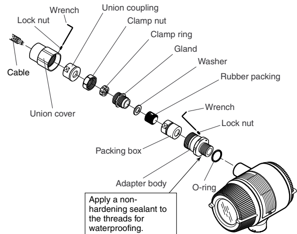
Figure 8.4.3 Installing Flameproof Packing Adapter
