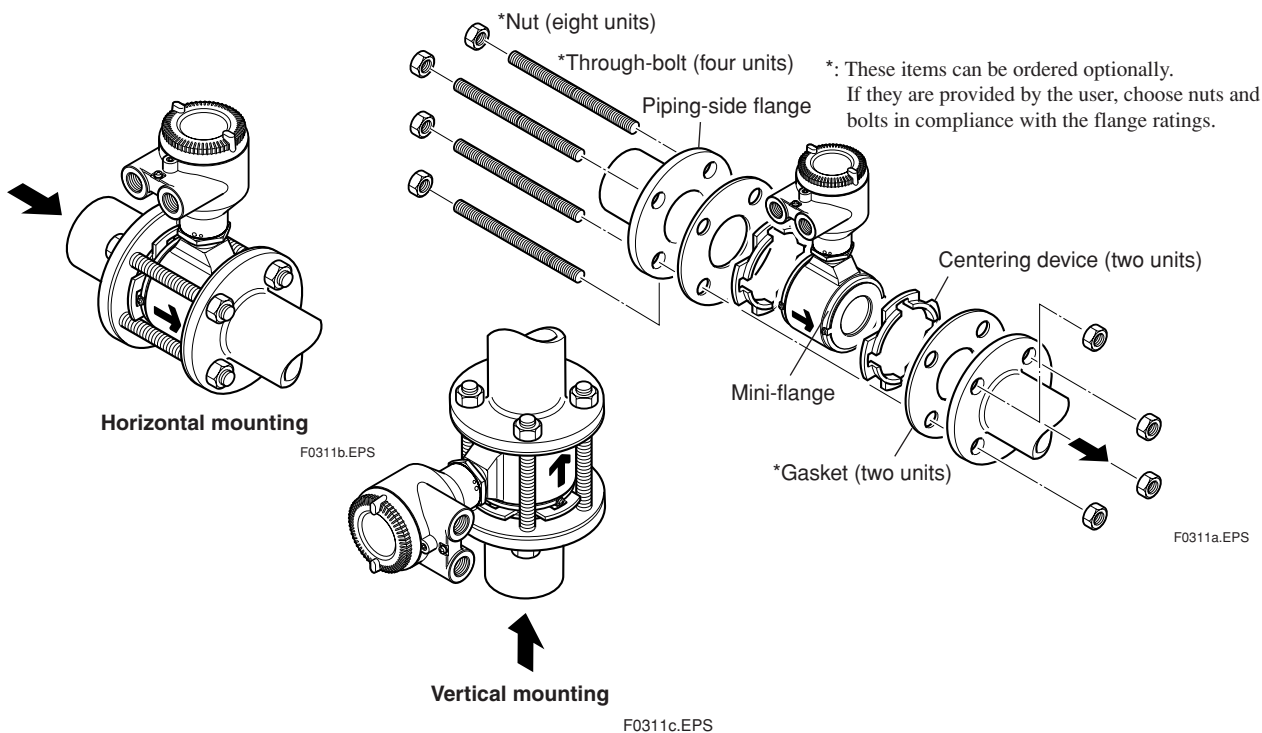
Figure 3.3.3 Mounting Procedure for Wafer Type (size: 25 mm (1.0 in.), 32 mm (1.25 in.), and 40 mm (1.5 in.))
