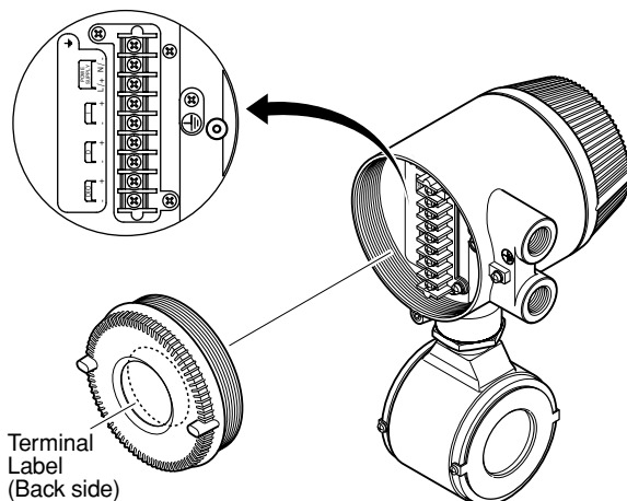
Figure 4.1.6 Terminal Configuration
