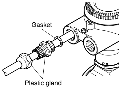
Figure 4.2.6 Plastic Gland (Optional code EP)
