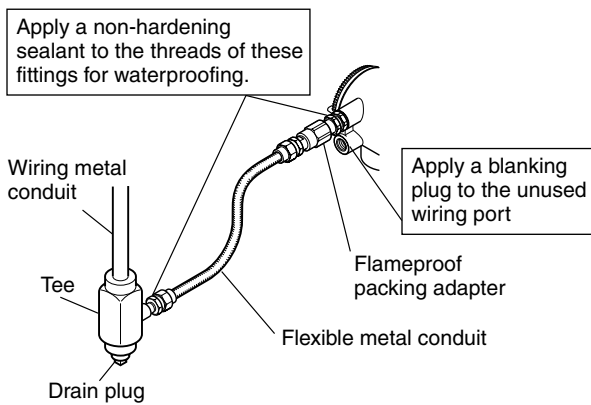
Figure 8.4.2 Typical Wiring Using Flexible Metal Conduit
