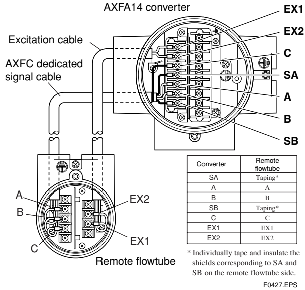
Figure 4.2.12 Wiring Diagram
