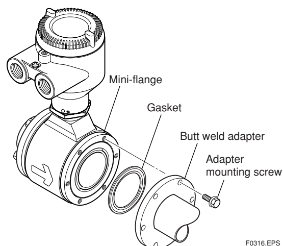
Figure 3.3.8 Mounting Procedure for Weld Joint Adapter Type
