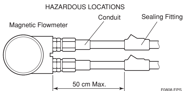
Figure 8.3 Conduit Wiring
