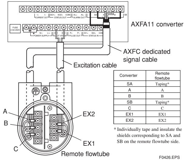
Figure 4.2.11 Wiring Diagram
