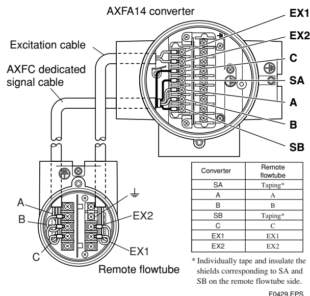
Figure 4.2.14 Wiring Diagram
