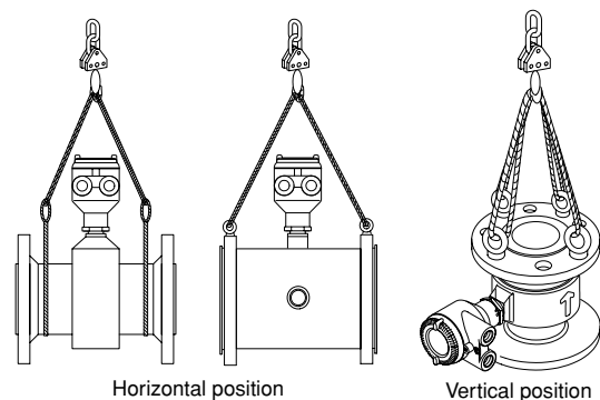
Figure 3.2.1 Lifting Flowmeter
