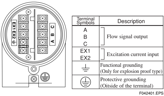
Figure 4.2.10 Terminal Configuration (Explosion proof Type)
