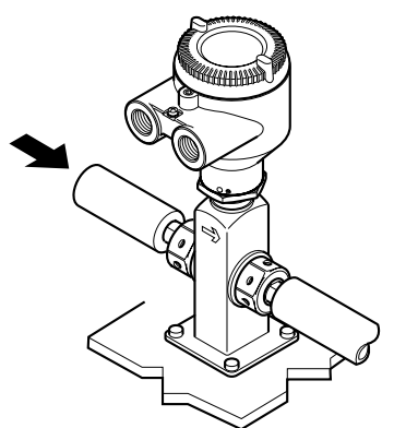
Horizontal mounting
