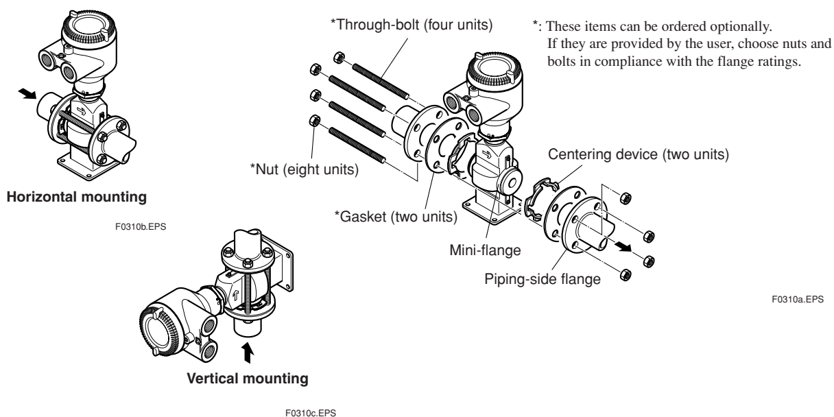
Figure 3.3.2 Mounting Procedure for Wafer Type (size: 2.5 mm (0.1 in.) to 15 mm (0.5 in.))
